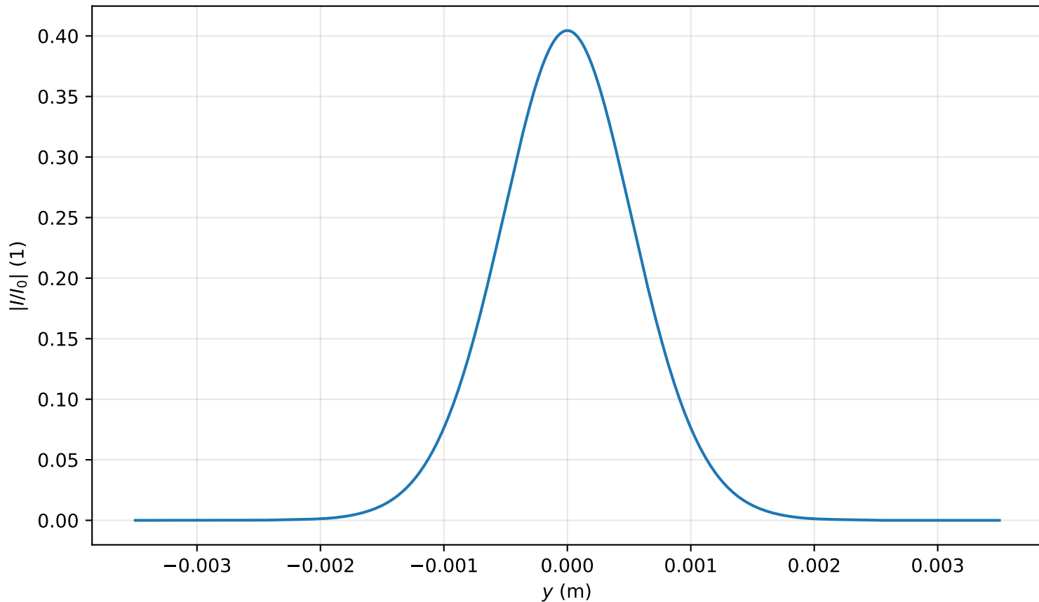
Intensity profile I(x=0, y, z=3.105)/I_0 , P_{in}=0.3P_{cr} , artificial time
